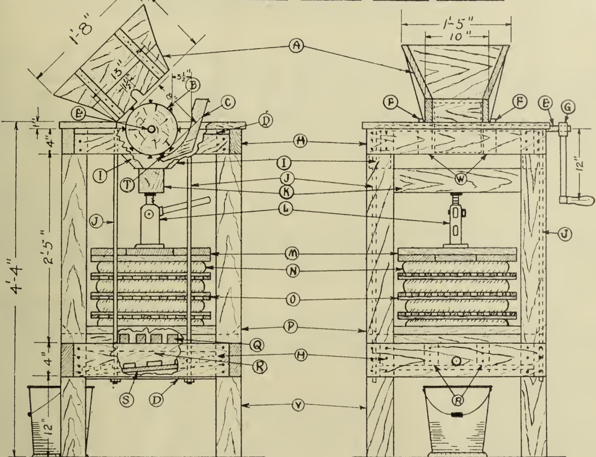
— SIDE ELEVATION —
